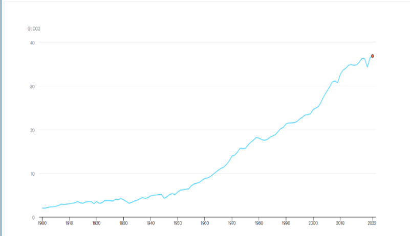
Global CO 2 emissions from energy combustion and industrial processes, 1900-2022
