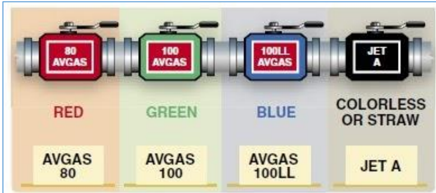
Figure 6-32. Aviation fuel color-coding system.
