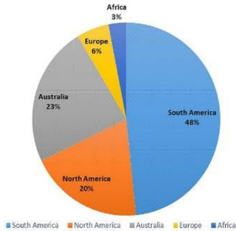
Availability of lithium in the World
