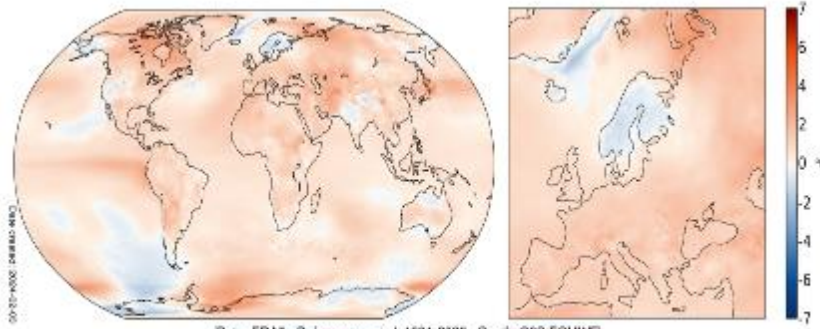
Surface air temperature anomaly for February 2023 to January 2024
