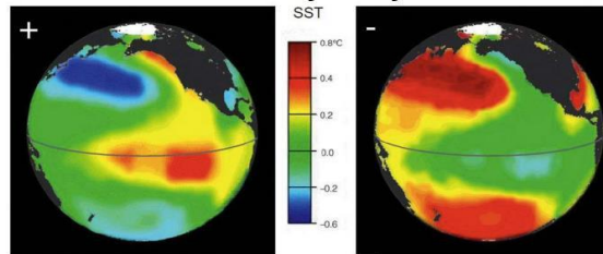
Positive PDO pattern
